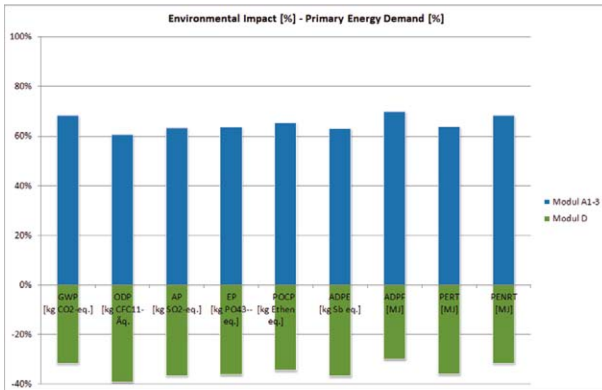
Impact categories for the life cycle of 1kg RHEINZINK-PROTECT®
